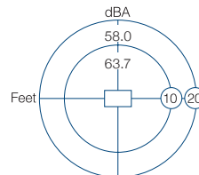
Generator at 100% rated load
